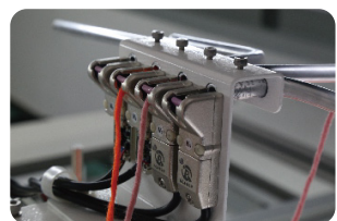
断线检测装置 Yarn Breakage Detection Device
